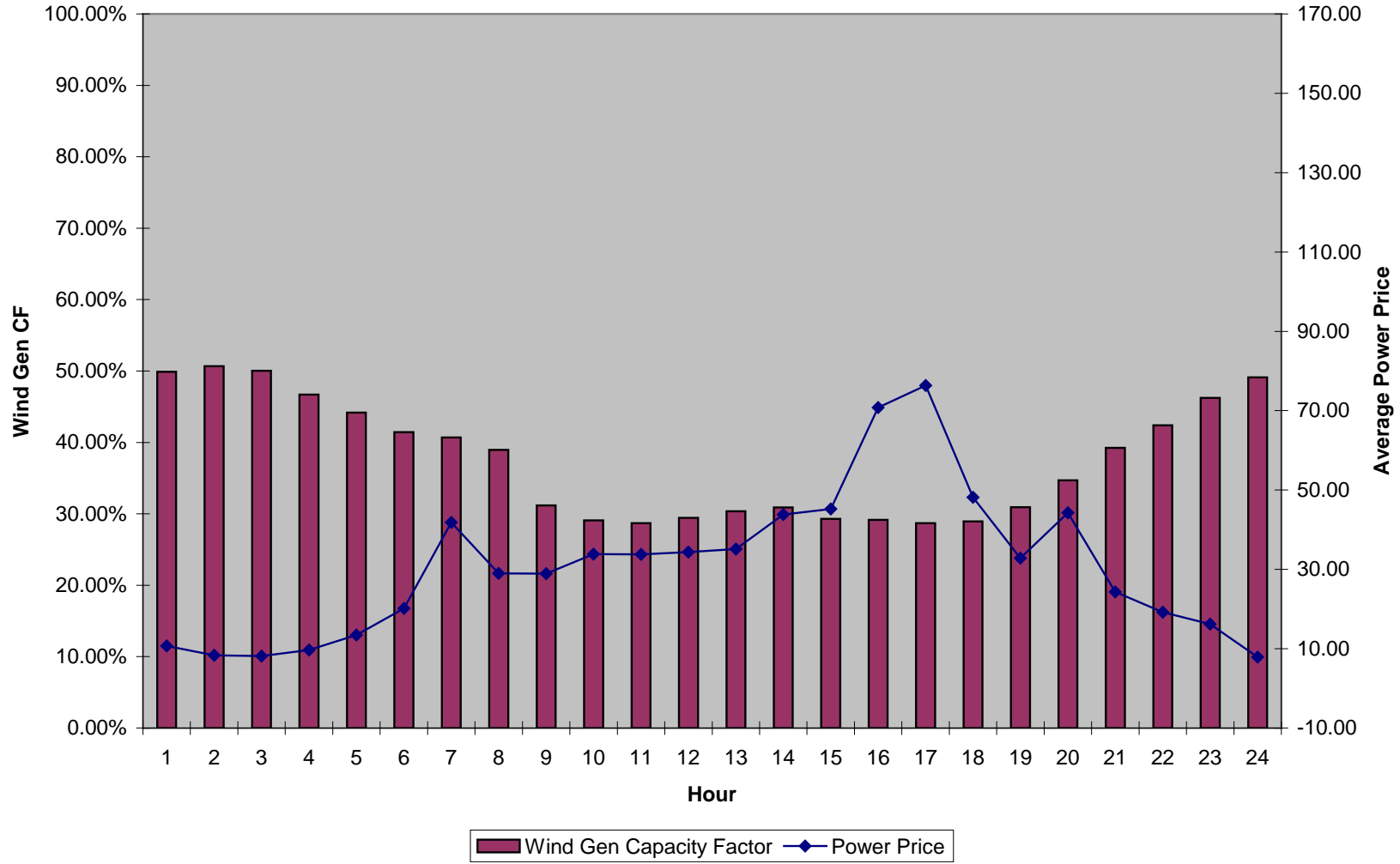
Wind Generation Capacity Factor and Power Price - October
