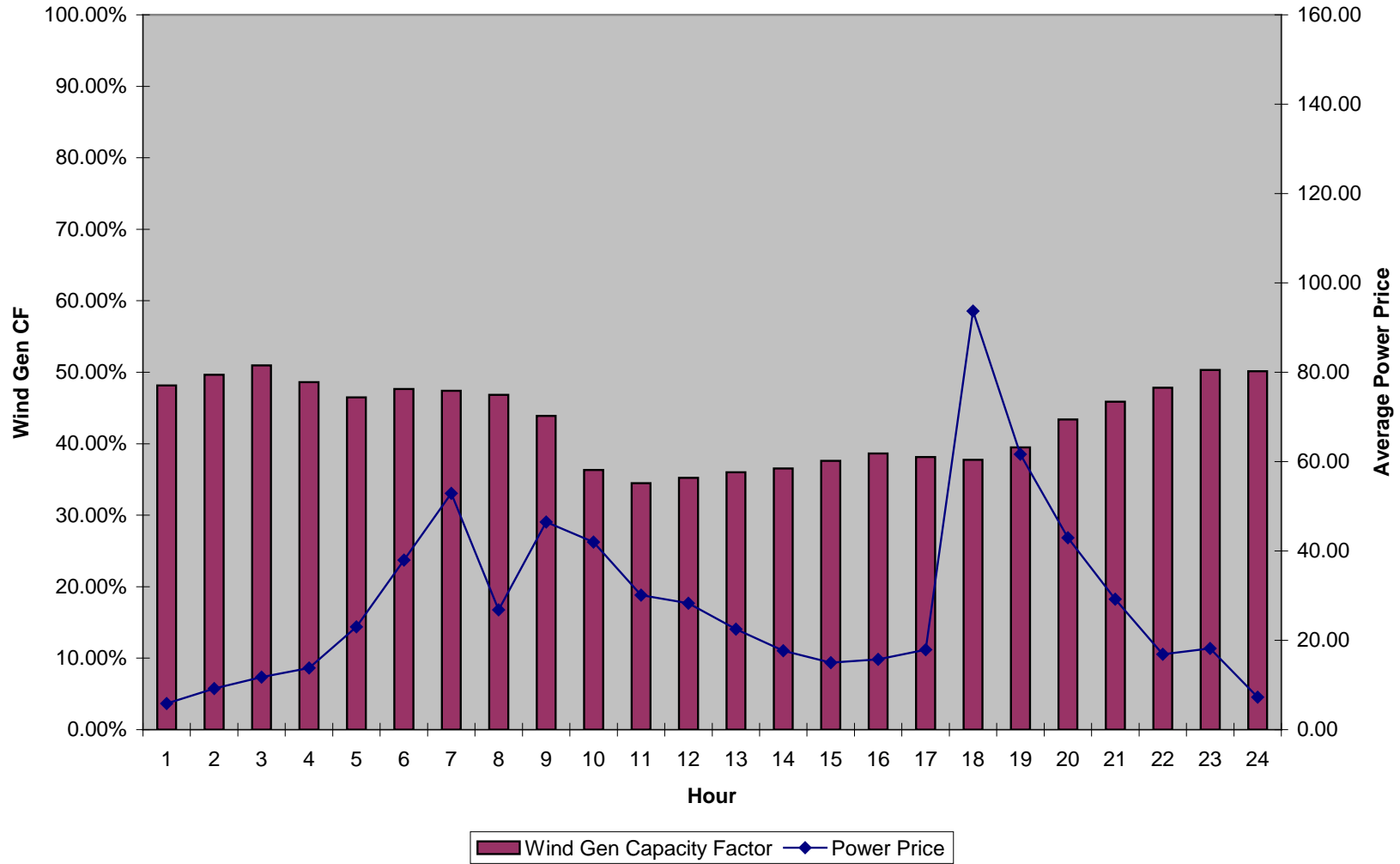
Wind Generation Capacity Factor and Power Price - December
