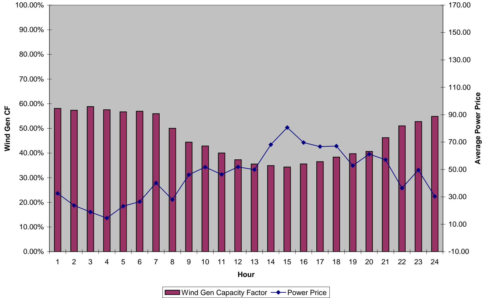
Wind Generation Capacity Factor and Power Price - April
