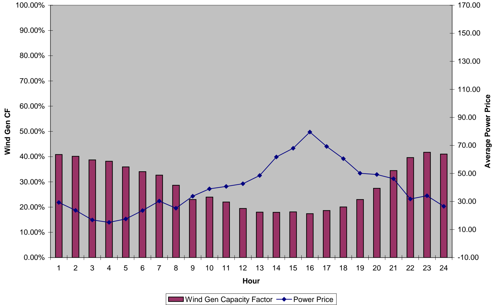
Wind Generation Capacity Factor and Power Price - September
