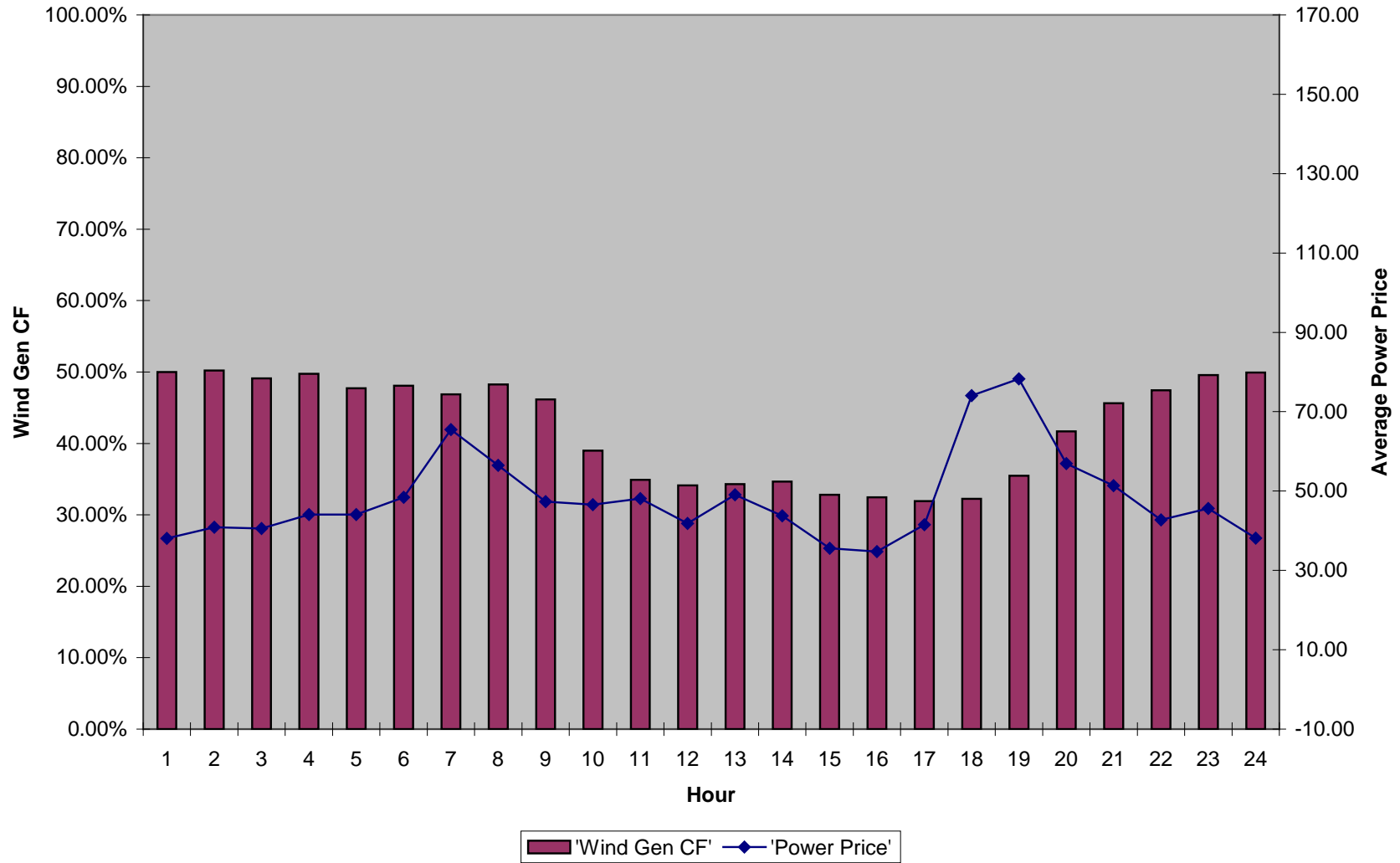
Wind Generation Capacity Factor and Power Price - January
