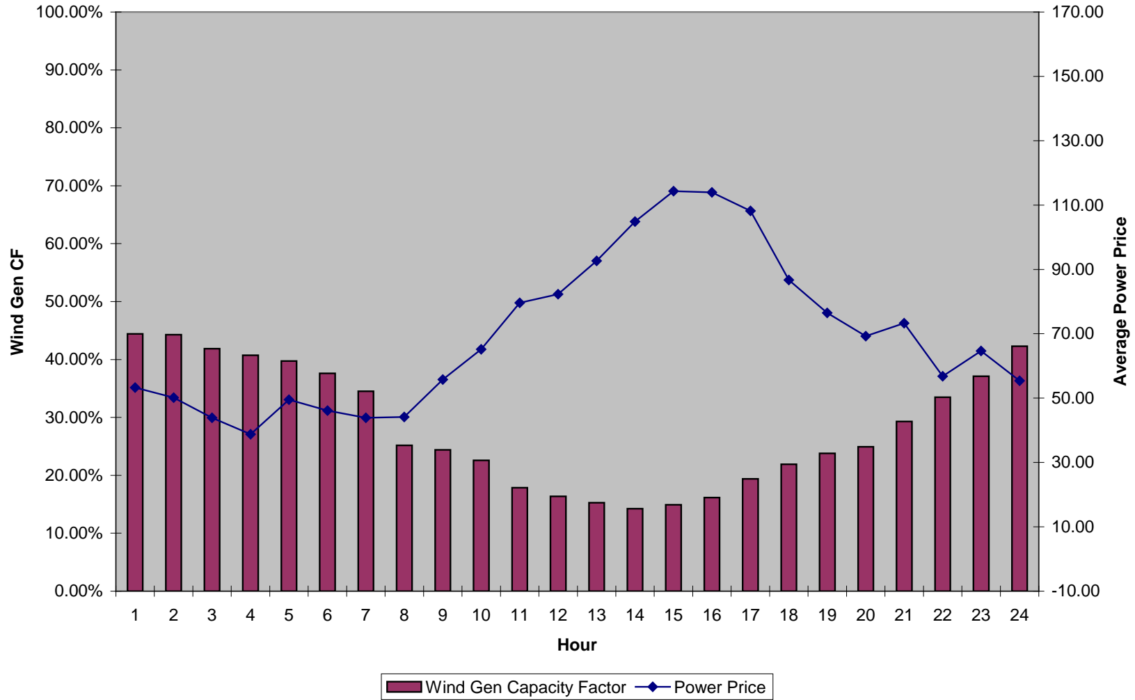
Wind Generation Capacity Factor and Power Price - August
