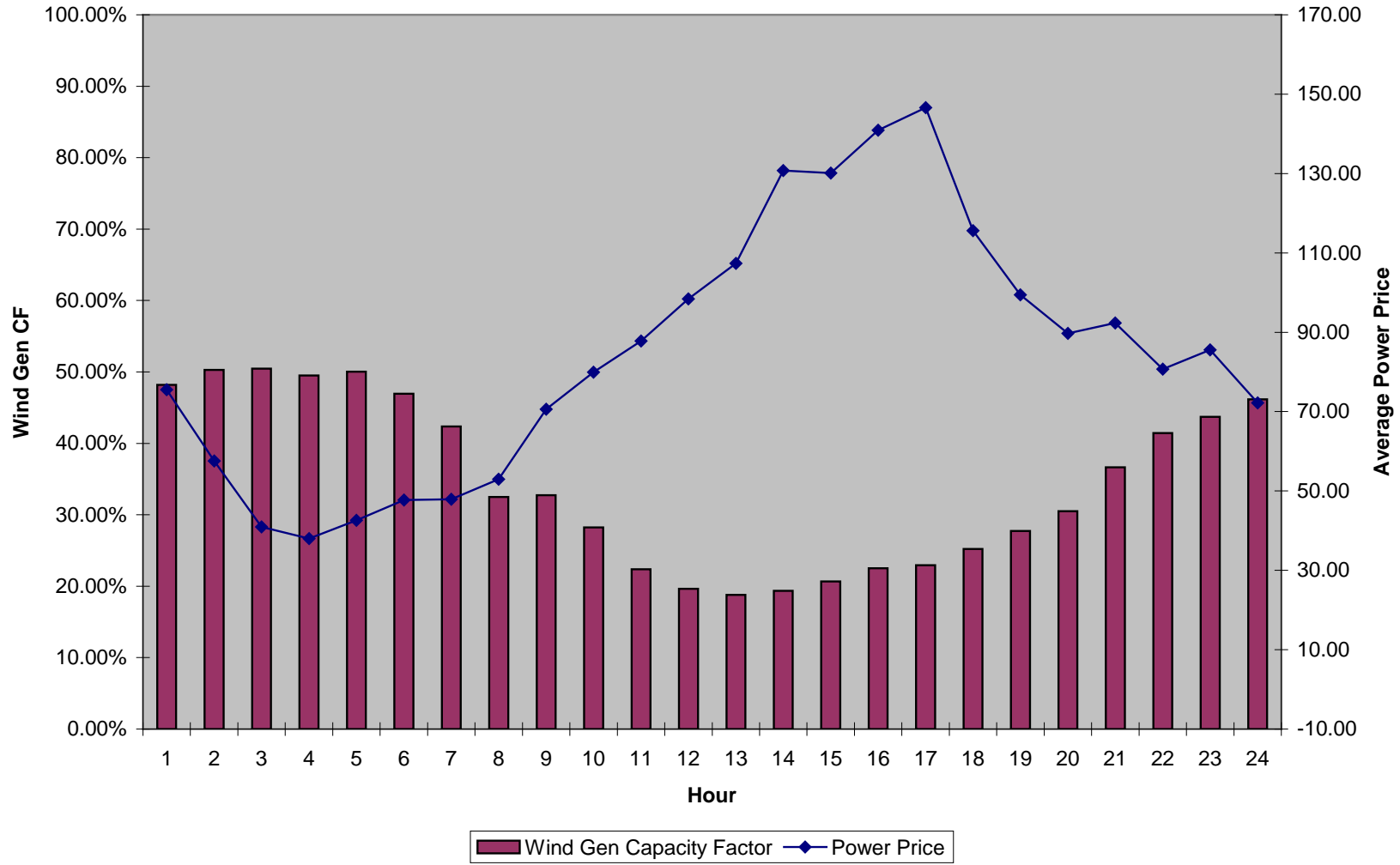
Wind Generation Capacity Factor and Power Price - July
