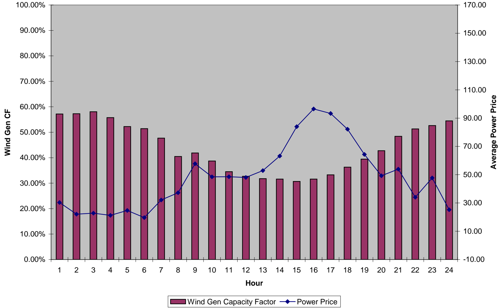
Wind Generation Capacity Factor and Power Price - May
