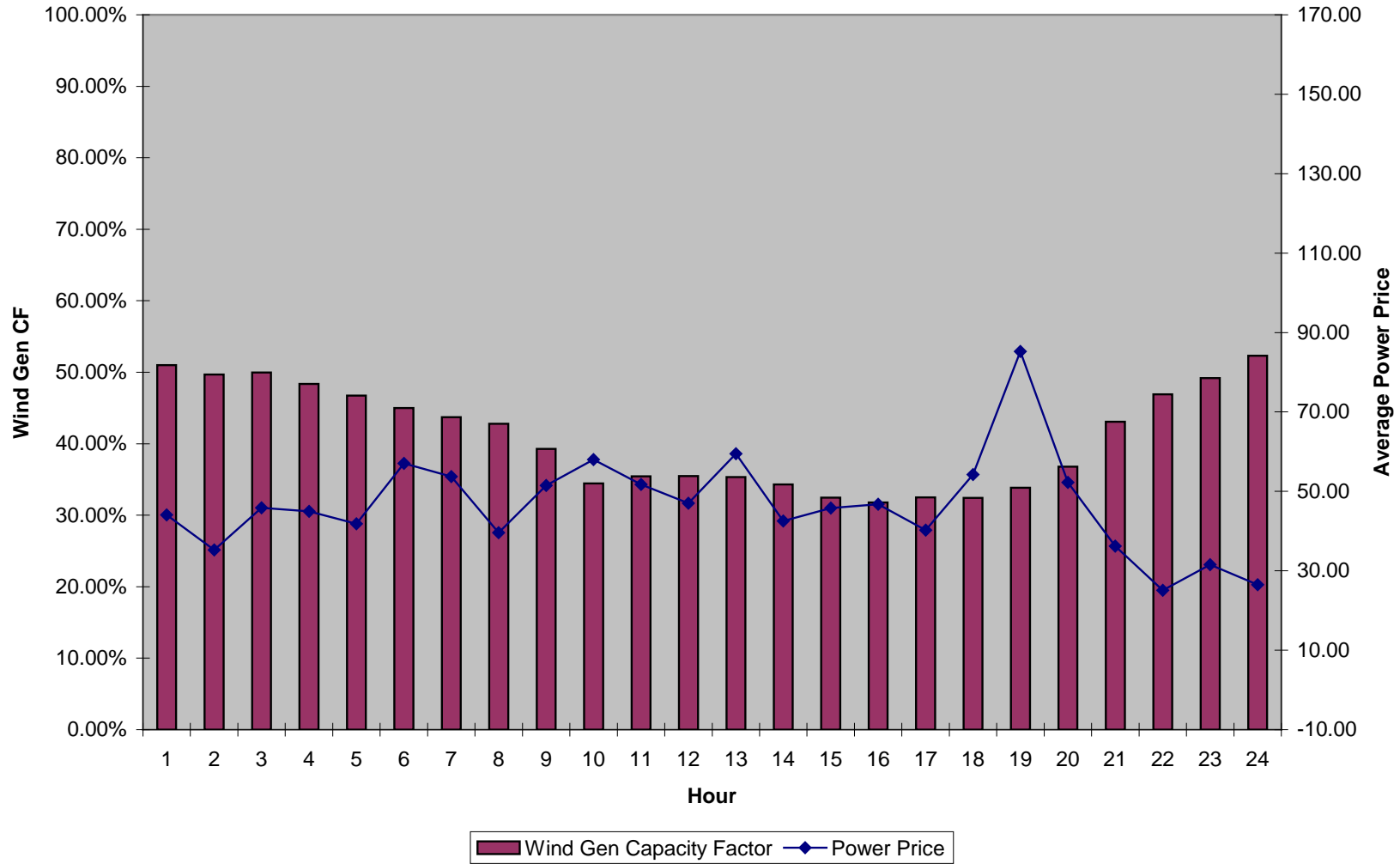
Wind Generation Capacity Factor and Power Price - February
