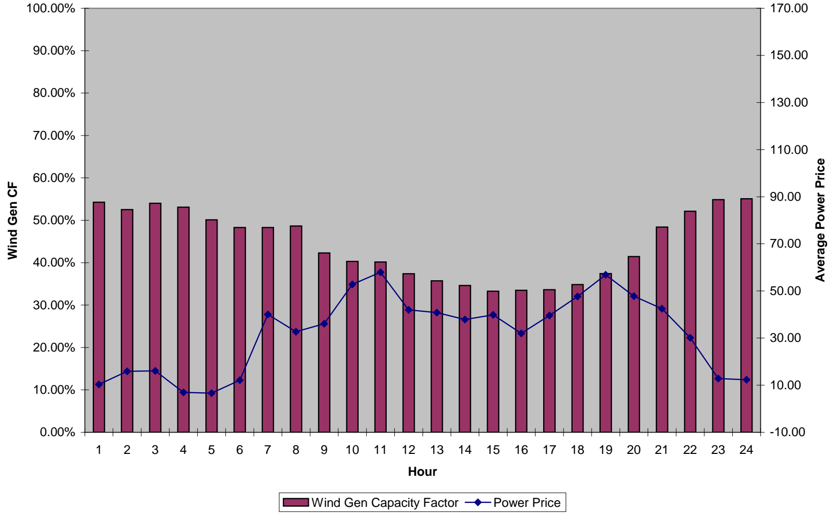
Wind Generation Capacity Factor and Power Price - March
